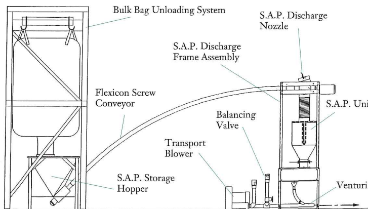
Remote Loading/Flex Screw Delivery
